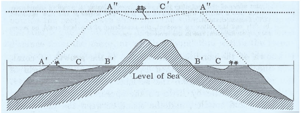
FIGURE 1.17. Darwin's explanation of coral reefs as shown in The Voyage of the Beagle . He explained that as the "new encircling barrier-reef" slowly sinks down, the corals continue to grow upward. The sea encroaches on the island until only the atoll remains ( dotted curve ).
