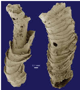
FIGURE 10.12. Phosphatized Cloudina specimens from the Neoproterozoic Dengying Formation in Shaanxi, China. Hard shelly parts appeared in metazoans during the Ediacaran, and the fossil on the right shows evidence of drilling predation.
