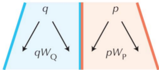
FIGURE 17.14. The ratios of allele frequencies q:p change in proportion to the fitnesses of the alleles, W_Q , W_P .
