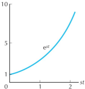
FIGURE 17.16. An allele with selective advantage s increases as \exp(st) or e^{st} while it is rare.
