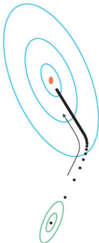
FIGURE 17.28. Correlations between traits will change the direction of the selection response, but will not prevent the population from reaching the optimum. The blue contours show mean fitness increasing toward an optimum ( red ). The green contours show the genetic variation for two traits, which are positively correlated. The dots show the evolution of this population toward the optimum, over more than 100 generations.
