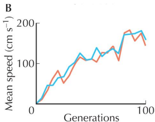
FIGURE 17.31. (A) Long-term selection for oil content in maize. (B) Selection on Drosophila for ability to fly upwind. The response to selection in two replicates is shown.
