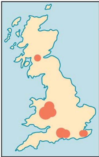
FIGURE 18.3. Resistance to the anticoagulant poison warfarin in rats ( Rattus norvegicus ) is due to multiple alleles. Areas where warfarin-resistant rats are found are in red. Here, resistant alleles are kept polymorphic by heterozygote advantage. The Scottish, Welsh, and English resistance outbreaks are due to different alleles.
