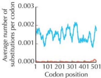
FIGURE 18.25. Synonymous ( blue ) and nonsynonymous ( red ) variation in the glycoprotein gene of vesicular stomatitis virus, an RNA virus that infects cattle. Variation is measured using a 20-bp sliding window. Overall, synonymous variation is 20 times higher.
