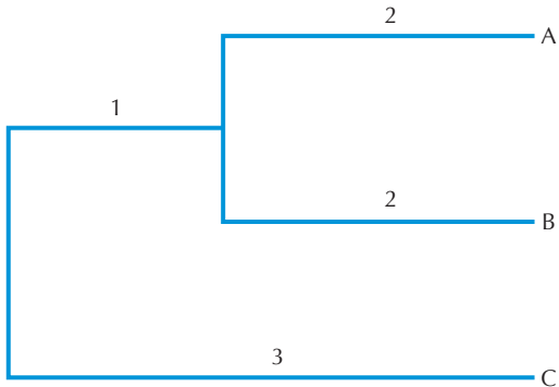
FIGURE 27.16. An ultrametric tree. (Redrawn from http://www.icp.ucl.ac.be/~opperd/private/upgma.html .)
