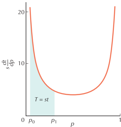
FIGURE 28.8. Plot of s(dt/dp) = 1/pq , the rate of time against allele frequency. The blue area under the curve is the total time taken to go from p_0 to p_1 .
