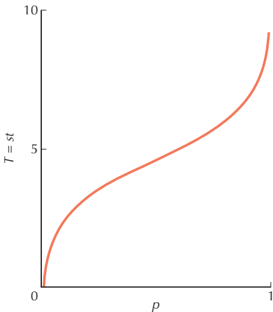
FIGURE 28.9. Plot of the integral of 1/pq , which is equal to s times the elapsed time (i.e., T = st ).
