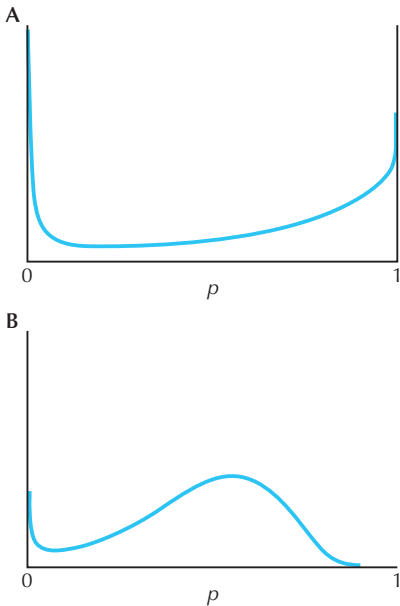
FIGURE 28.27. The distribution of allele frequencies under migration, selection, and drift; p^* = 0.05 . (A) Nm = 0.25 , Ns = 1 . (B) Nm = 2 , Ns = 4 .
