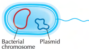
FIGURE 6.4. ( Top ) Bacterial plasmids. ( Middle ) Lysed bacterial DNA. ( Bottom ) Cartoon of a bacterial cell with a circular chromosome and a circular plasmid. (The DNA is not drawn to scale.)
