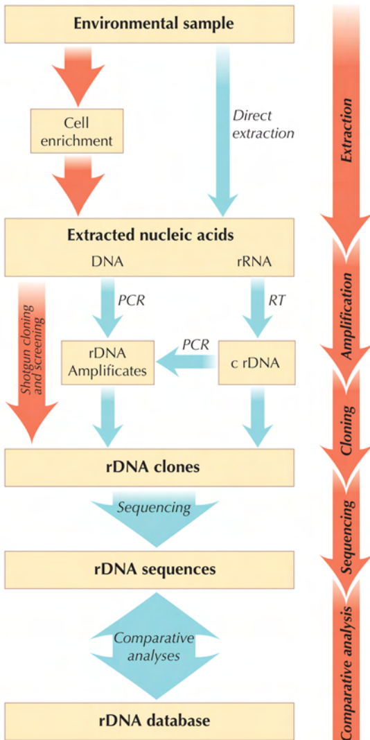
FIGURE 6.13. A flowchart illustrating the methods available for characterizing an environmental sample using rRNA sequence analysis. RT, reverse transcriptase.
