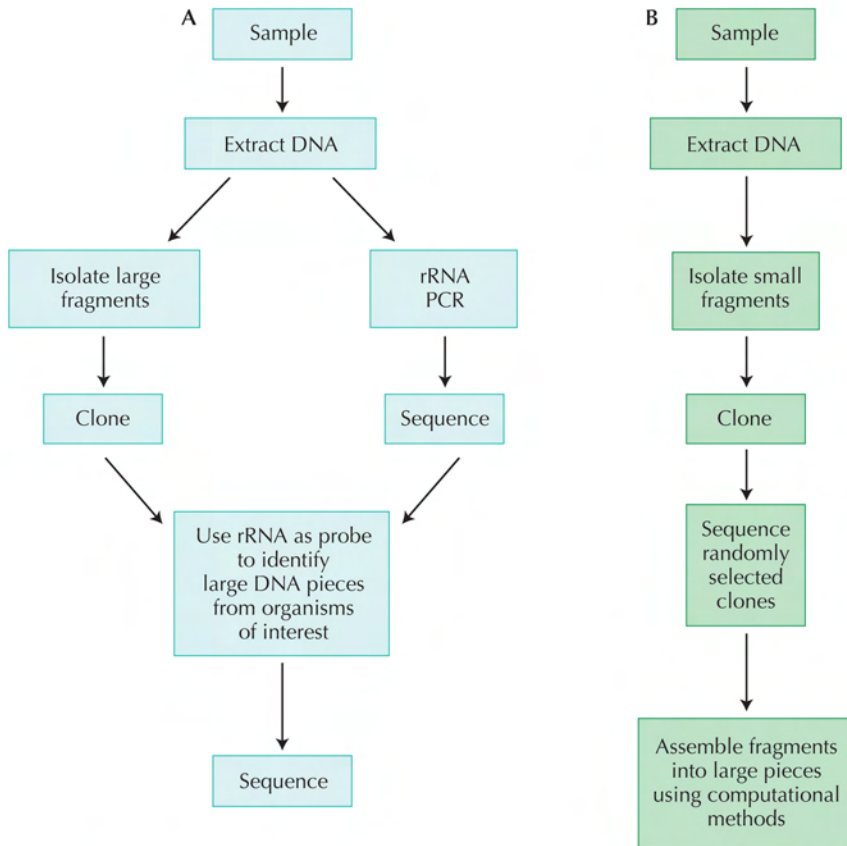
FIGURE 6.15. Methods used in metagenomics. (A) Phylogenetic anchor method. (B) Environmental shotgun sequencing.
