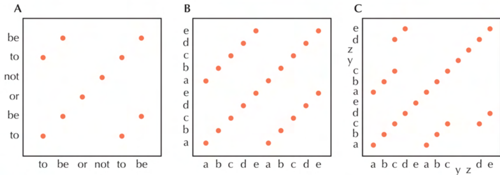
FIGURE 7.8. Dotplots of repeating text.
