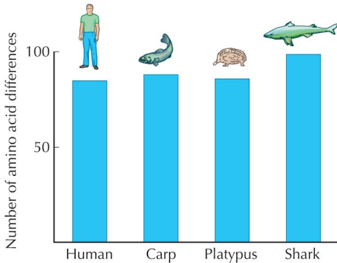
FIGURE 13.27. Comparisons between the \alpha - and \beta -globin genes show that the molecular clock ticks steadily; that is, divergence occurs at almost the same rate in different lineages.
