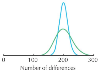
FIGURE 13.30. The blue curve shows the distribution of the number of differences between two sequences, given that the expected number is 200 and the actual number follows a Poisson distribution. The green curve shows a distribution with four times the Poisson variance. Even with this increased variance in rate, the molecular clock is roughly steady.
