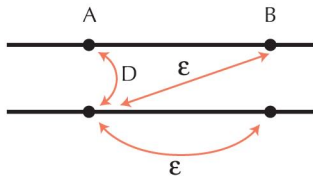
FIGURE 14.8. Dominance is an interaction between homologous genes at the same locus ( D ), whereas epistasis is an interaction between genes at different loci ( \epsilon ). Lines show the two genomes in a diploid individual, with loci A, B.
