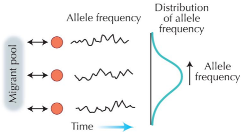
FIGURE 16.7. In the island model, demes exchange genes with a pool of migrants ( left ). Allele frequencies in individual demes fluctuate at random over time ( middle ), but the population as a whole reaches a steady statistical distribution ( right ).
