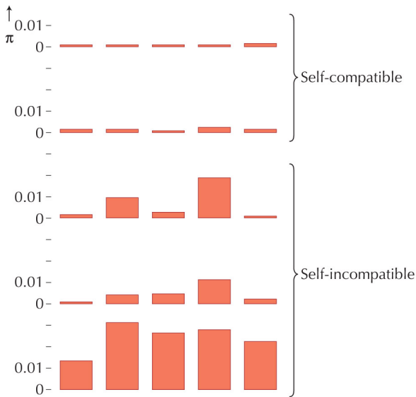
FIGURE 19.20. Diversity in self-fertilizing species tends to be lower than in their outcrossing relatives. This example shows levels of nucleotide diversity at silent sites, \pi , around five genes, sampled from five species of wild tomato. The three self-incompatible species are much more diverse than the two self-compatible species.
